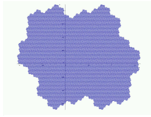
Fig. 2: Rauzy fractal for the Tribonacci number
