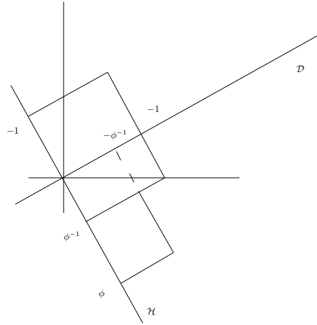
Fig. 1: Generalized Rauzy fractal for the Fibonacci number
